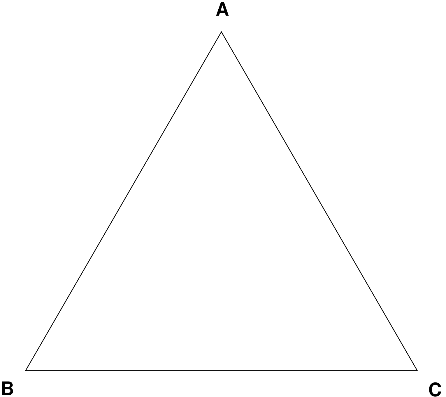
EQUILATERAL TRIANGLE
