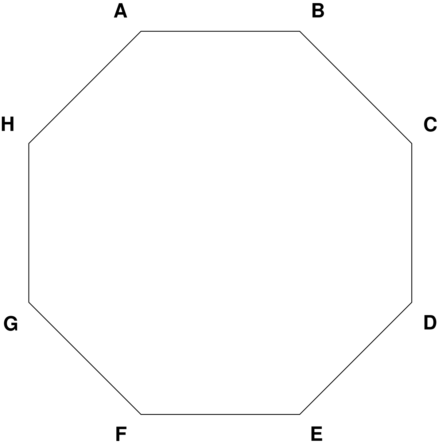
OCTAGON
